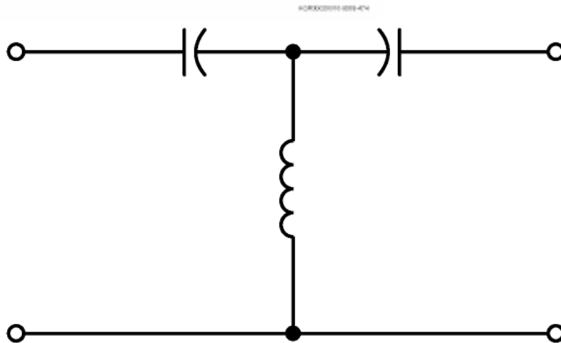
T-Type High Pass
