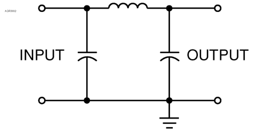
Pi-Type Low Pass
